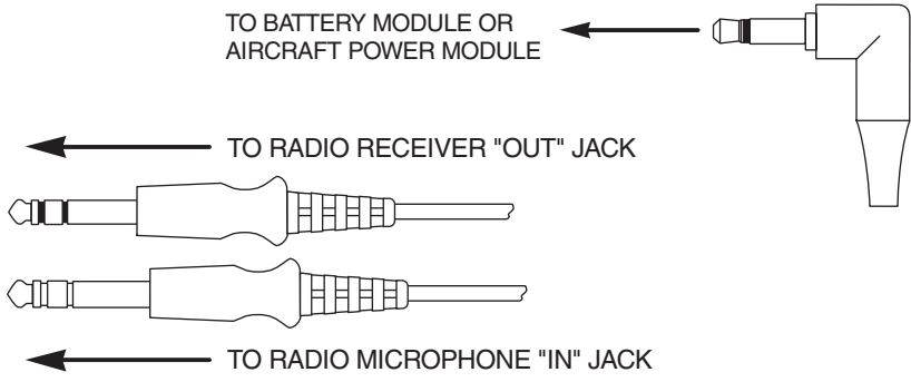
Figure 2: Connections
