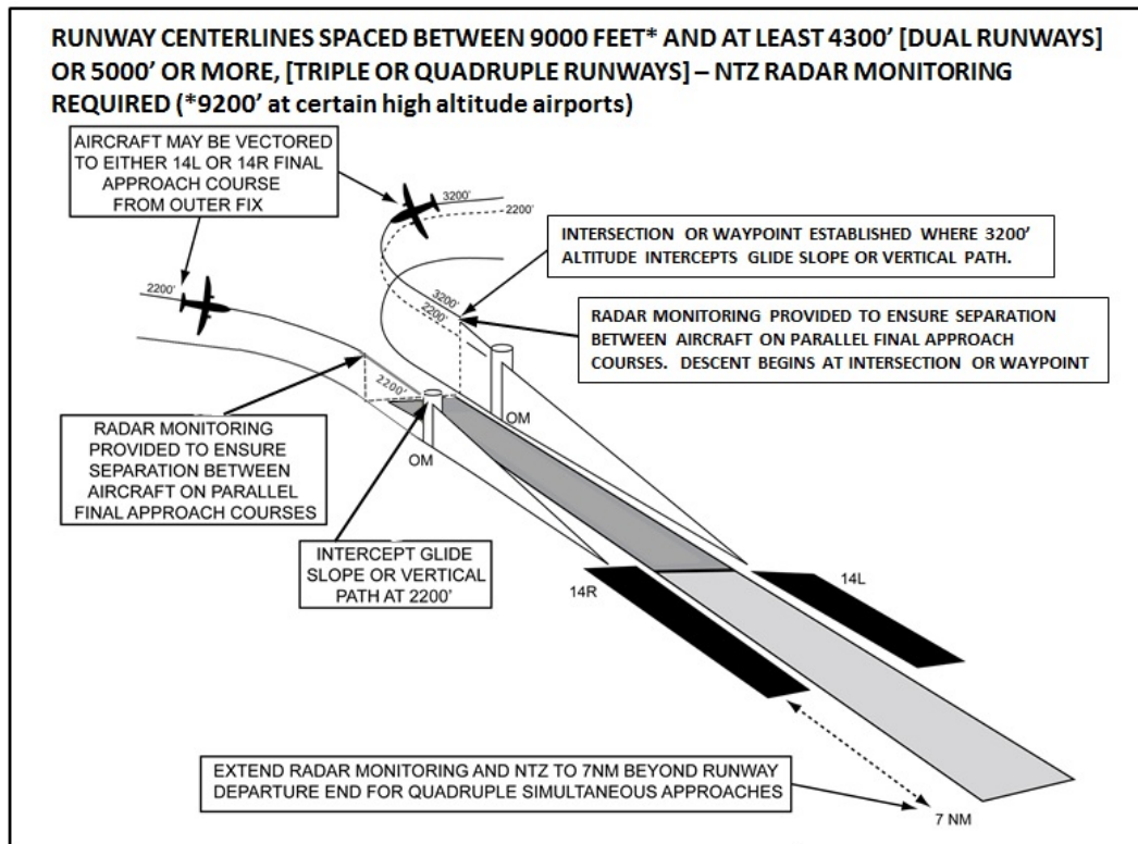
FIG 5-4-21 Simultaneous (Parallel) Independent ILS/RNAV/GLS Approaches
