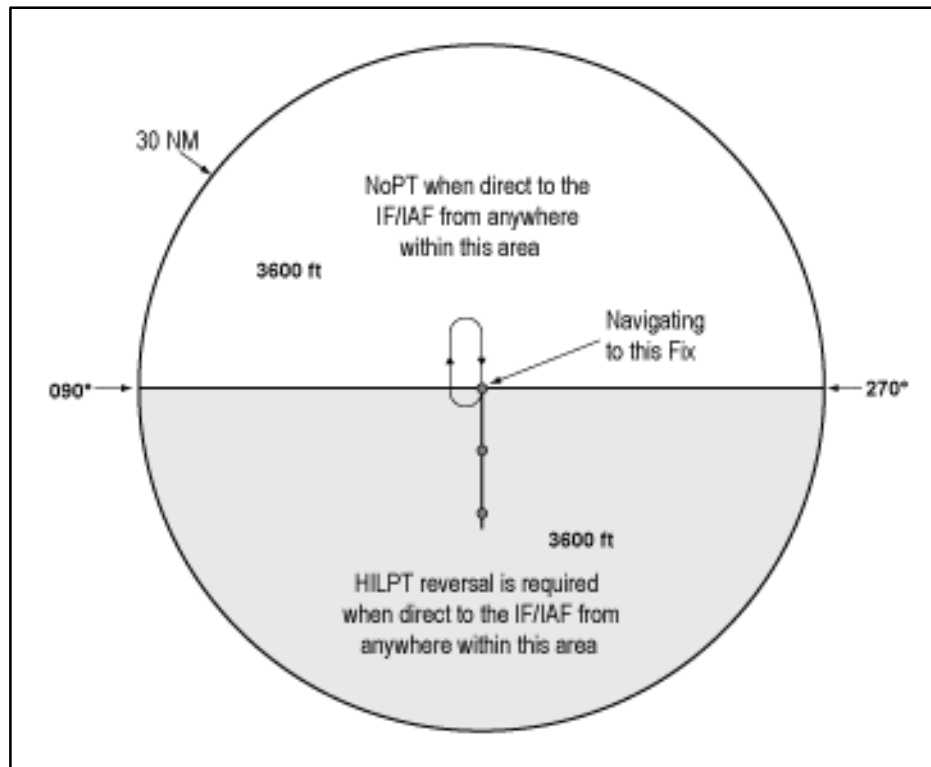
FIG 5-4-6 TAA with Left and Right Base Areas Eliminated
