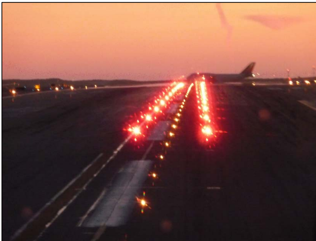
FIG 2-1-13 Takeoff Hold Lights
