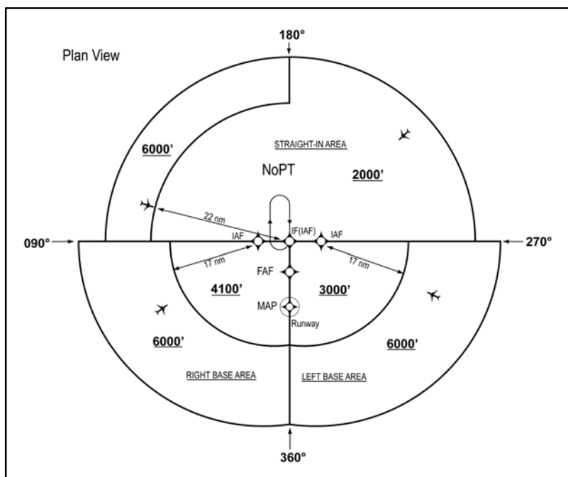
FIG 5-4-4 Sectored TAA Areas
