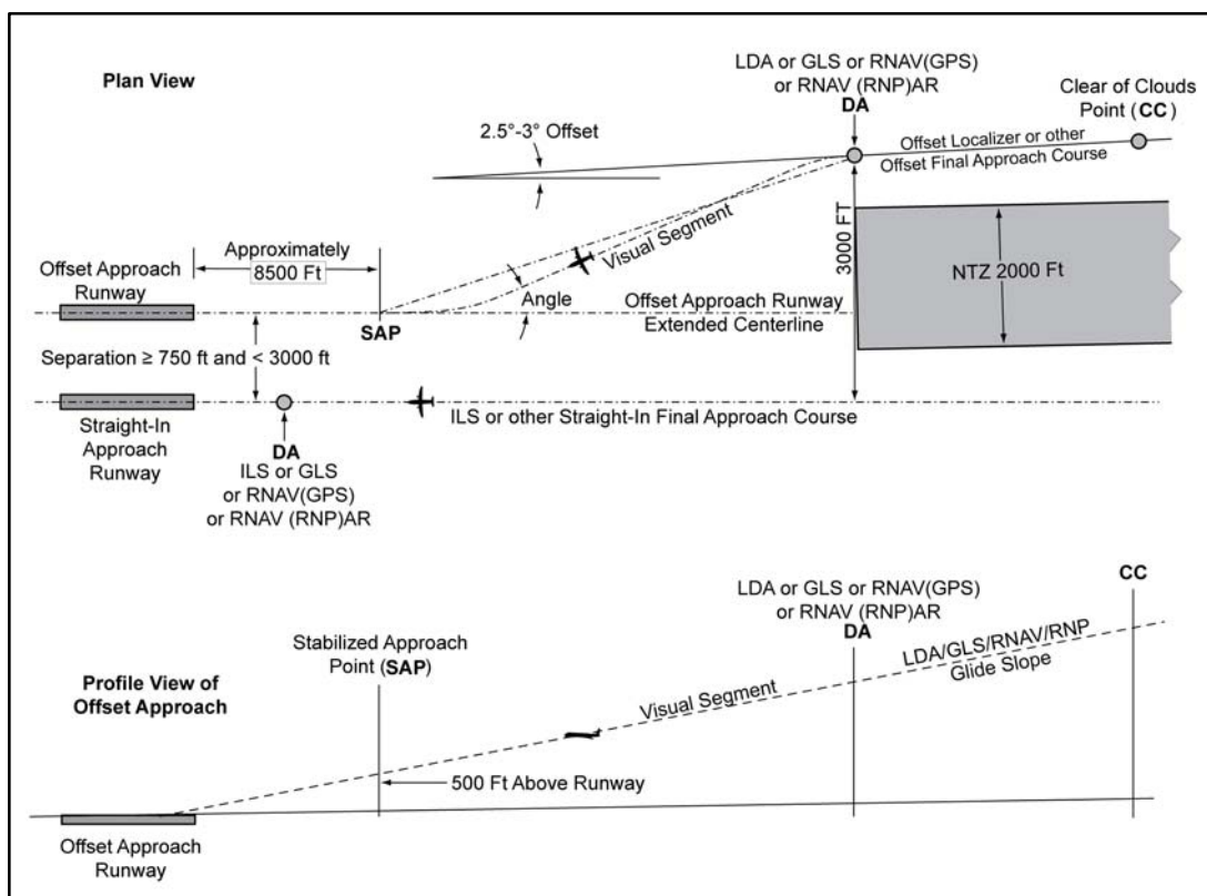
FIG 5-4-23 SOIA Approach Geometry
