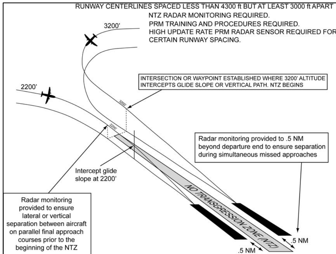
FIG 5-4-22 PRM Approaches Simultaneous Close Parallel
