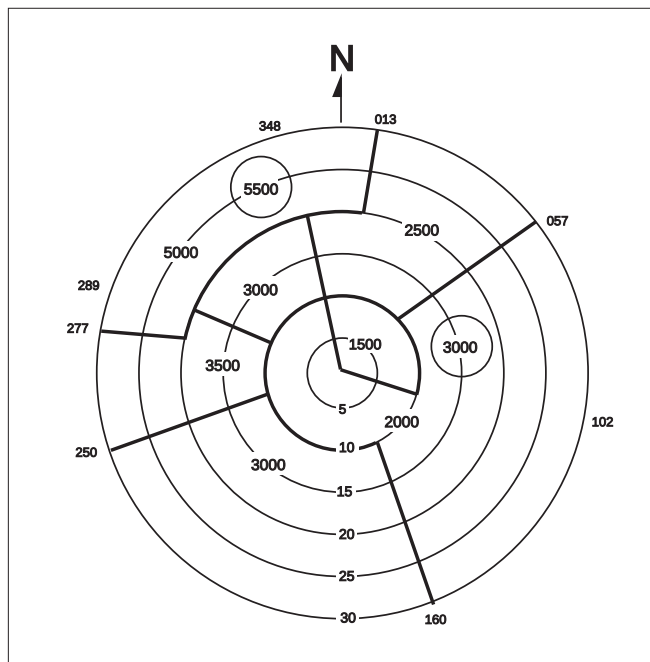
FIG 5-4-10 Minimum Vectoring Altitude Charts
