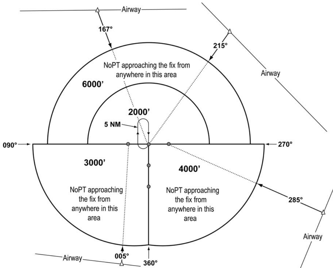
FIG 5-4-9 Examples of a TAA with Feeders from an Airway
