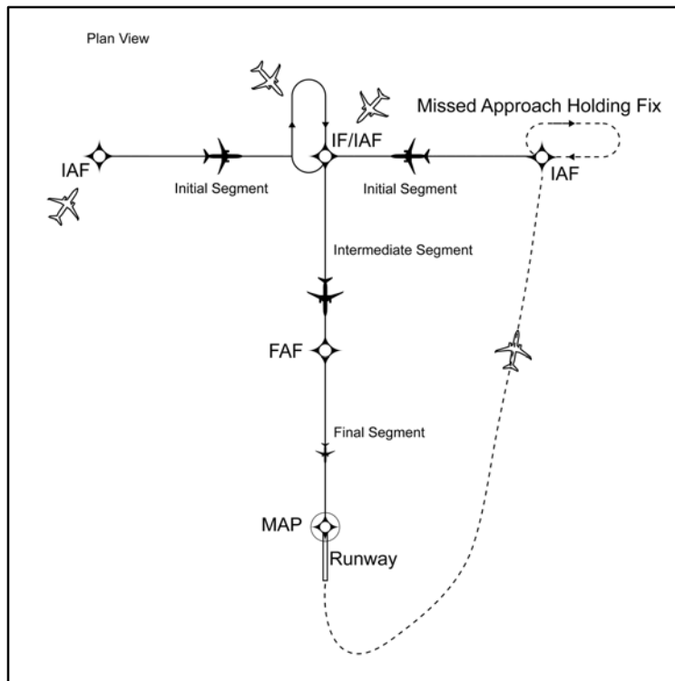
FIG 5-4-2 Basic “T” Design
