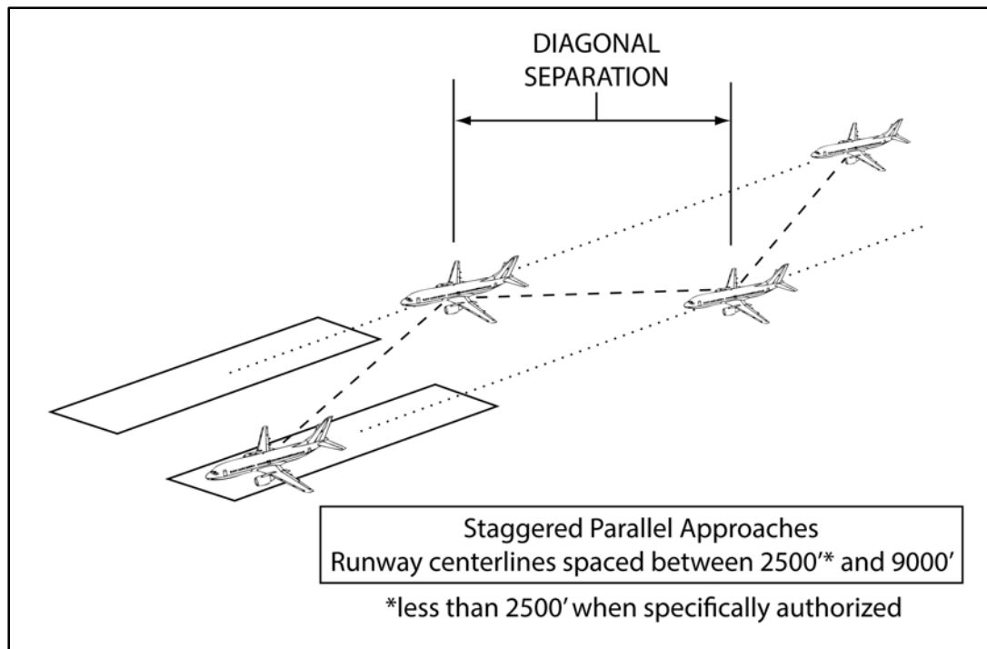
FIG 5-4-20 Simultaneous (Parallel) Dependent Approaches
