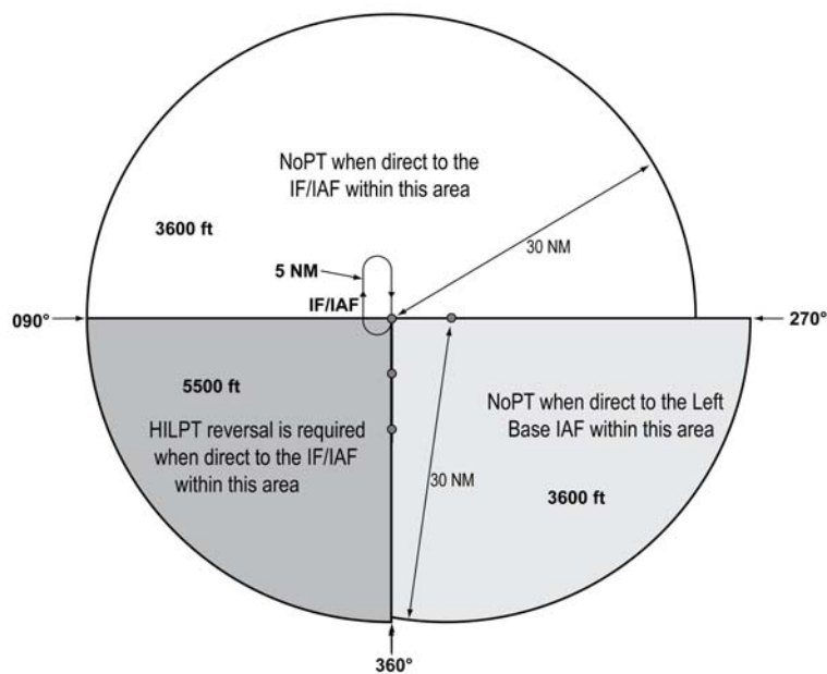
FIG 5-4-8 TAA with Right Base Eliminated
